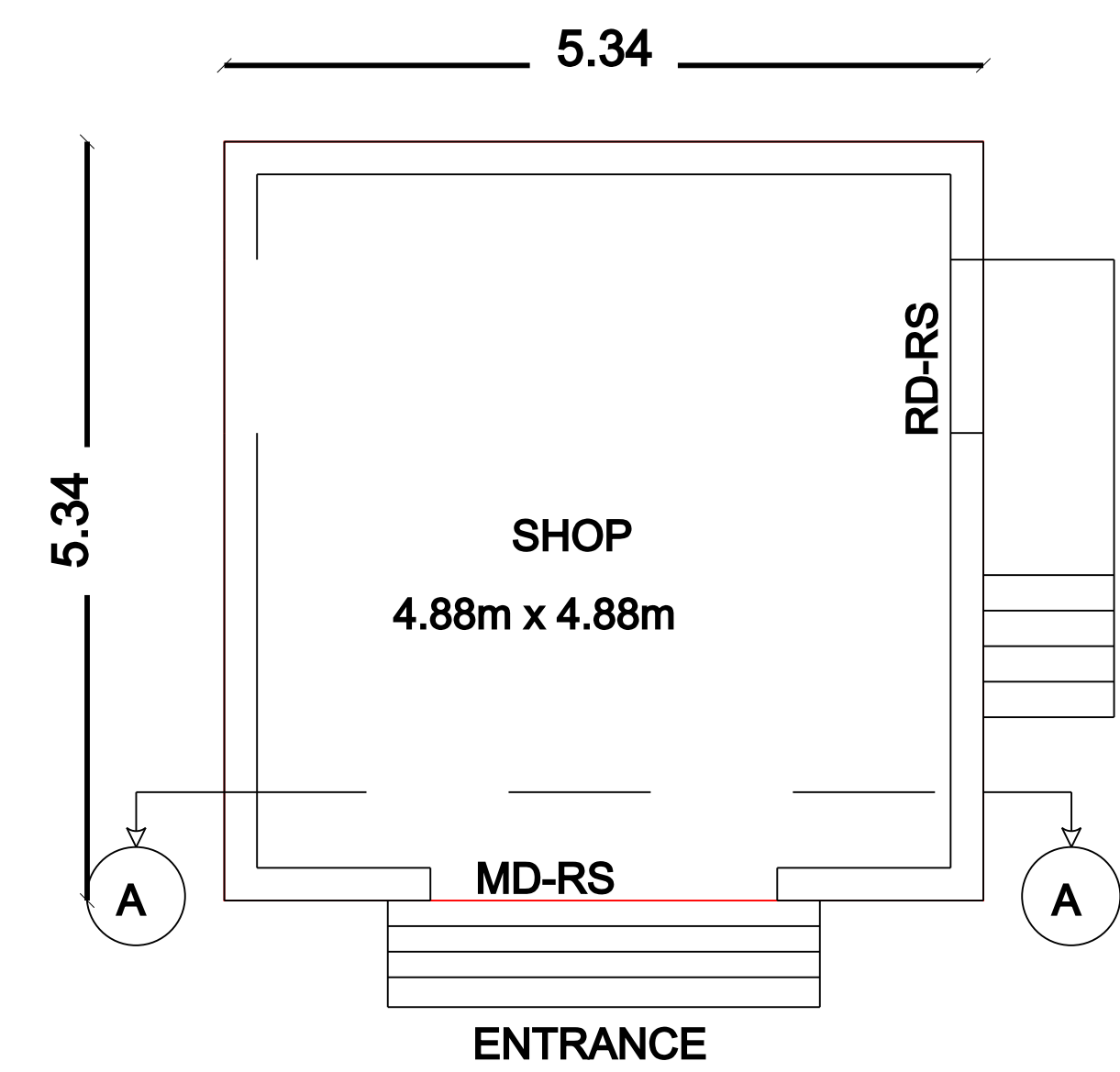
FLOOR PLAN
