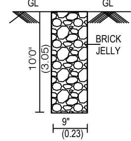
PERCOLATION PIT:-
