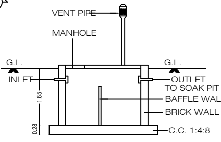
SECTION OF SEPT. TANK
