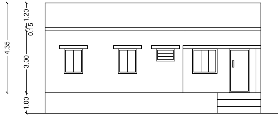
ELEVATION - EAST SIDE
