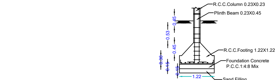
DETAILS OF COLUMN FOOTING (SCALE 1:50)
