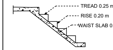
STAIR DETAILS
