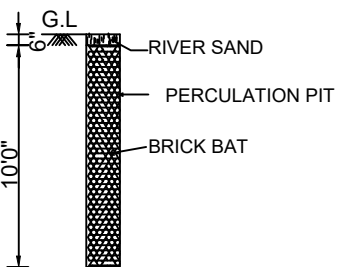
PERCOLATION PIT
