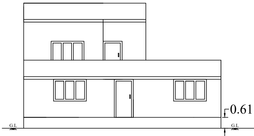
FRONT ELEVATION
