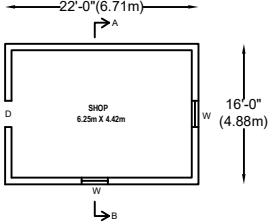
PROPOSED GROUND FLOOR
