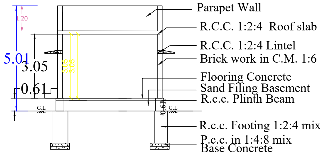
SECTION -"AB"
