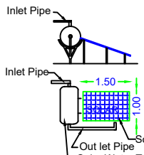
DETAILS OF SOLAR WATER HEATER
