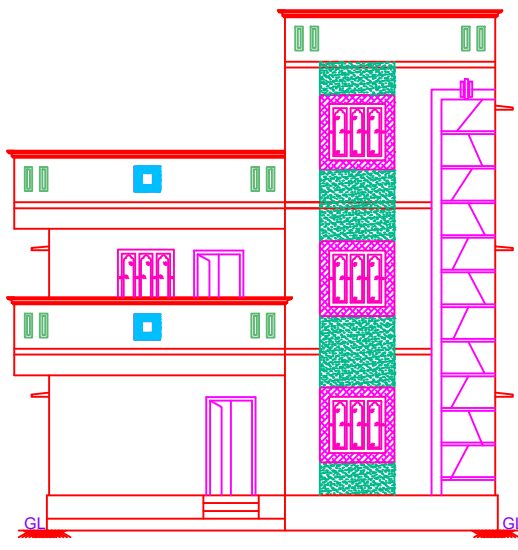
FRONT ELEVATION
