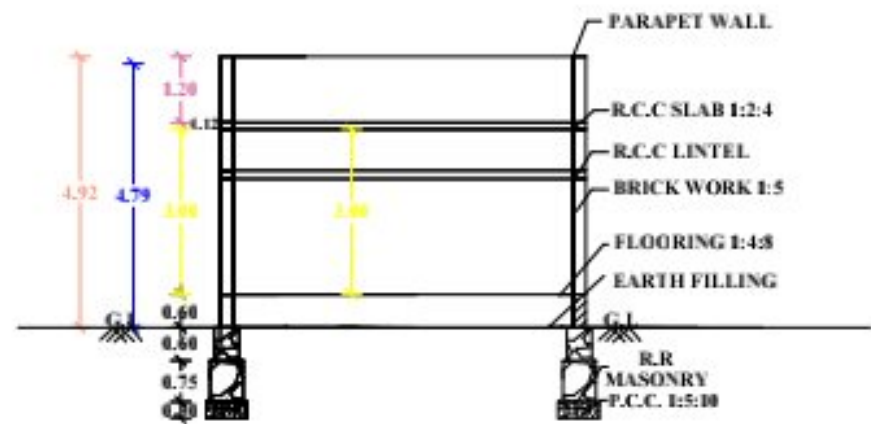
"SECTION 'AB'"
