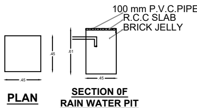
SECTION OF RAIN WATER PIT
