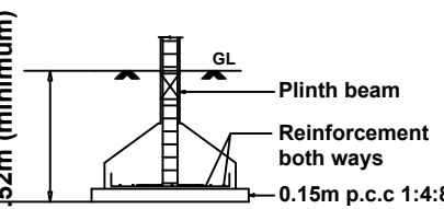
TYP.DET.COLUMN FOOTING
