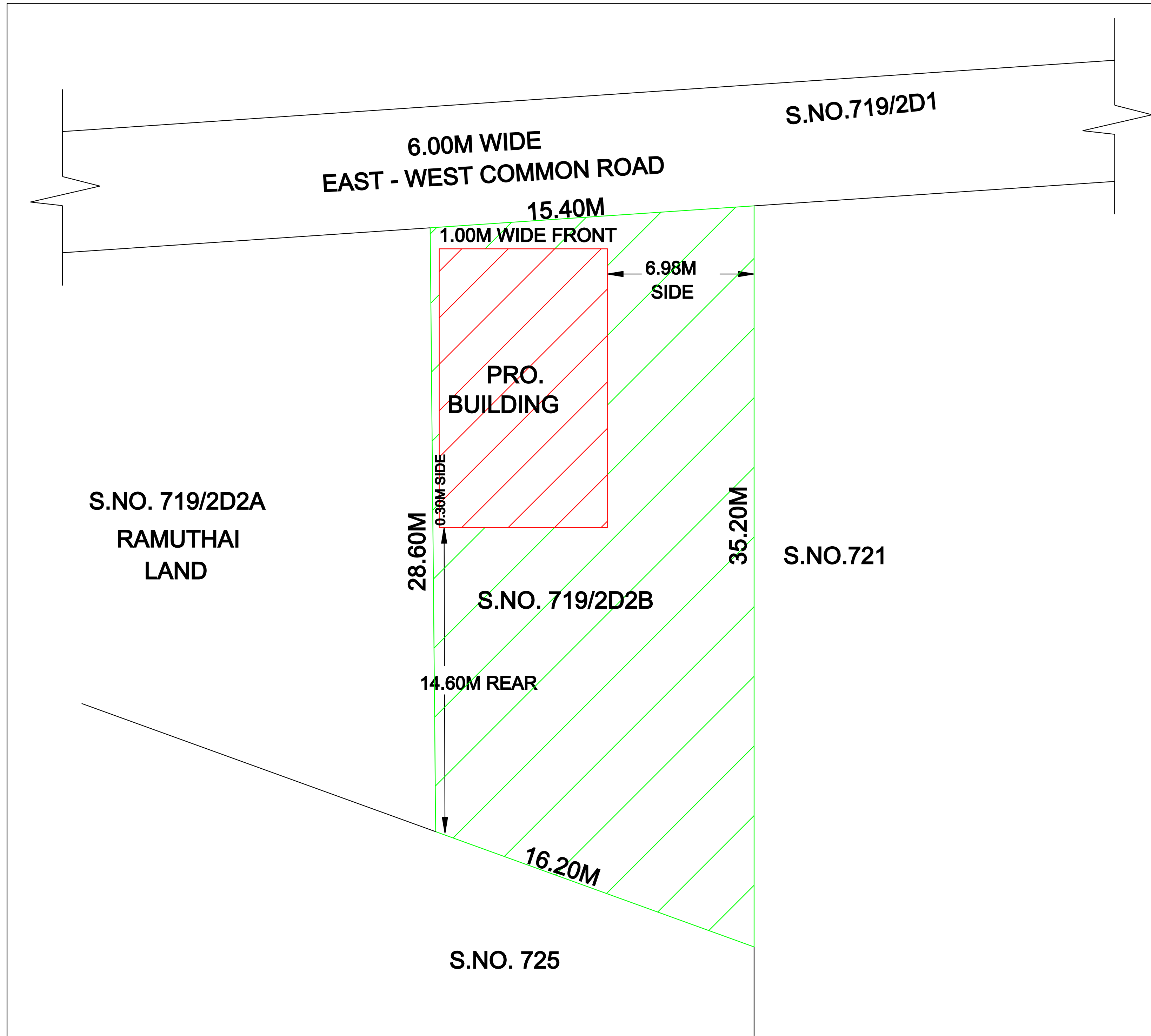
LOCATION PLAN
