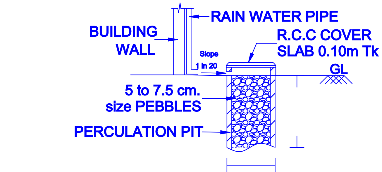
RAIN WATER HARVESTING TRENCH PIT DETAILS
