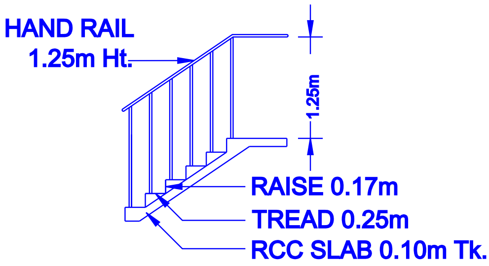
STEPS DETAILS
