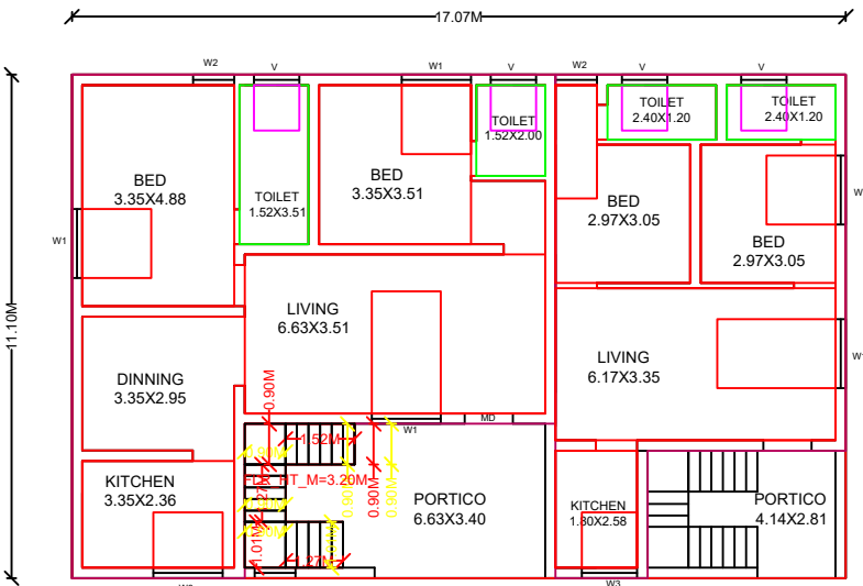
FLOOR PLAN
