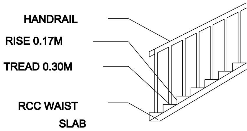
STAIRCASE
