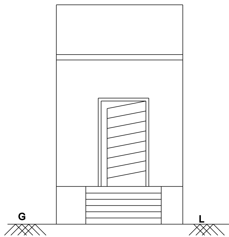
FRONT ELEVATION
