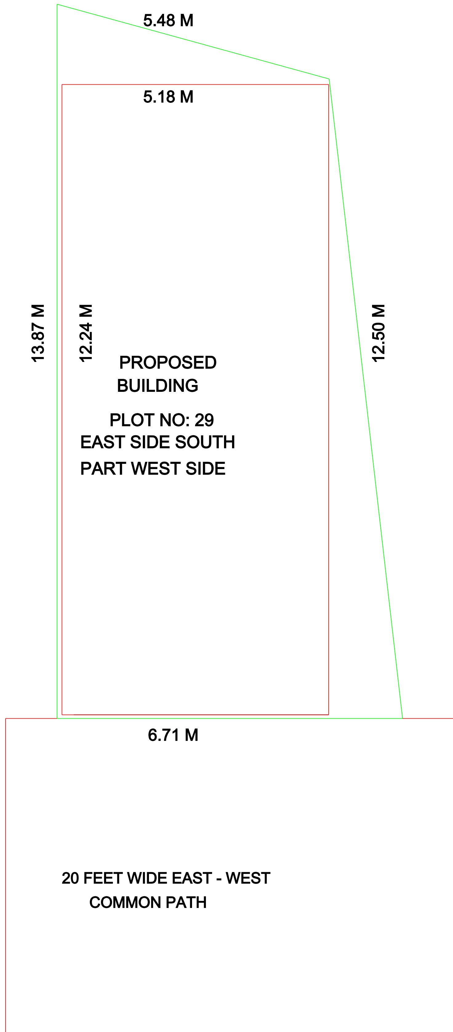
SITE PLAN
