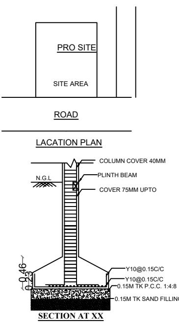
SECTION AT XX
