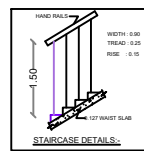
STAIRCASE DETAILS
