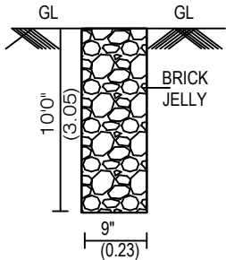
PERCULATION PIT:-
