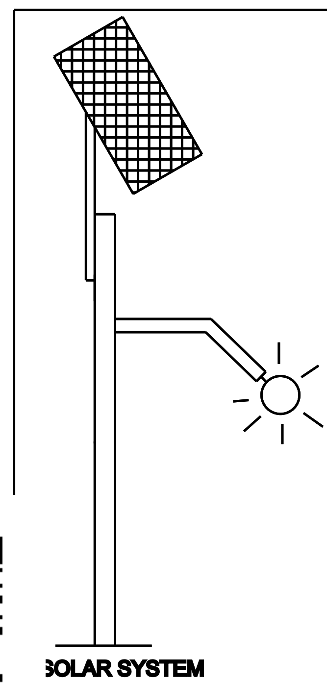
SOLAR SYSTEM
