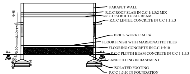
SECTION AB
