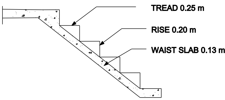
STAIR DETAILS
