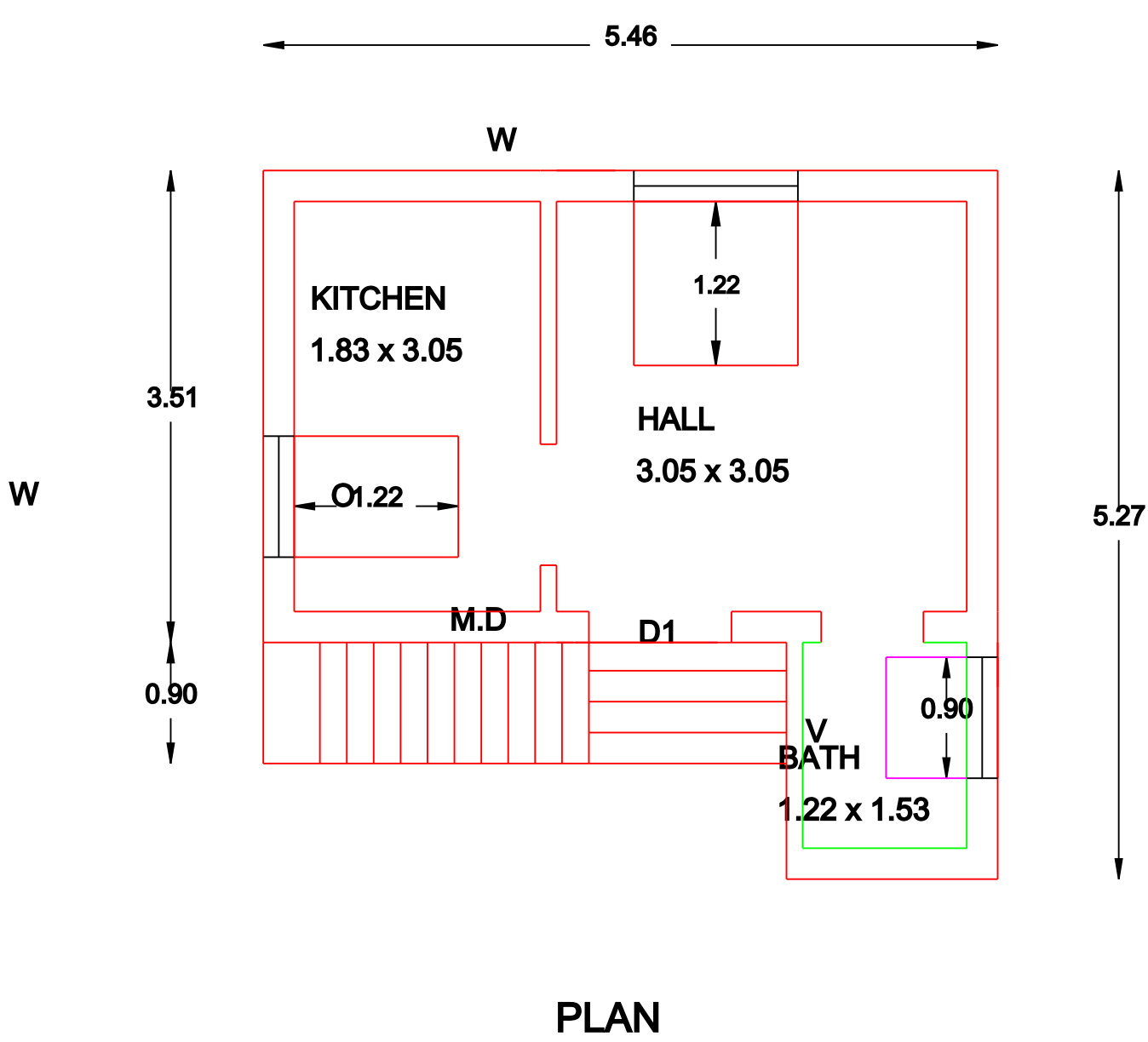
PLAN
