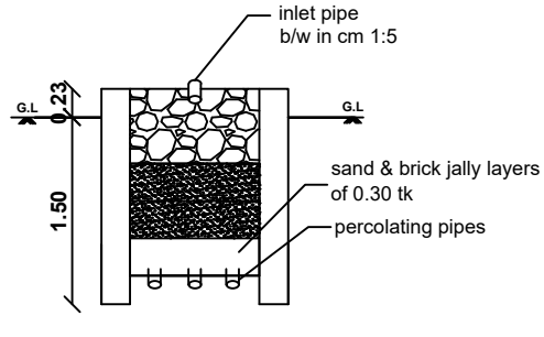
SECTION OF RAIN WATER HARVESTING PIT
