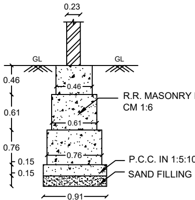
FOUNDATION DETAIL (NOT TO SCALE)
