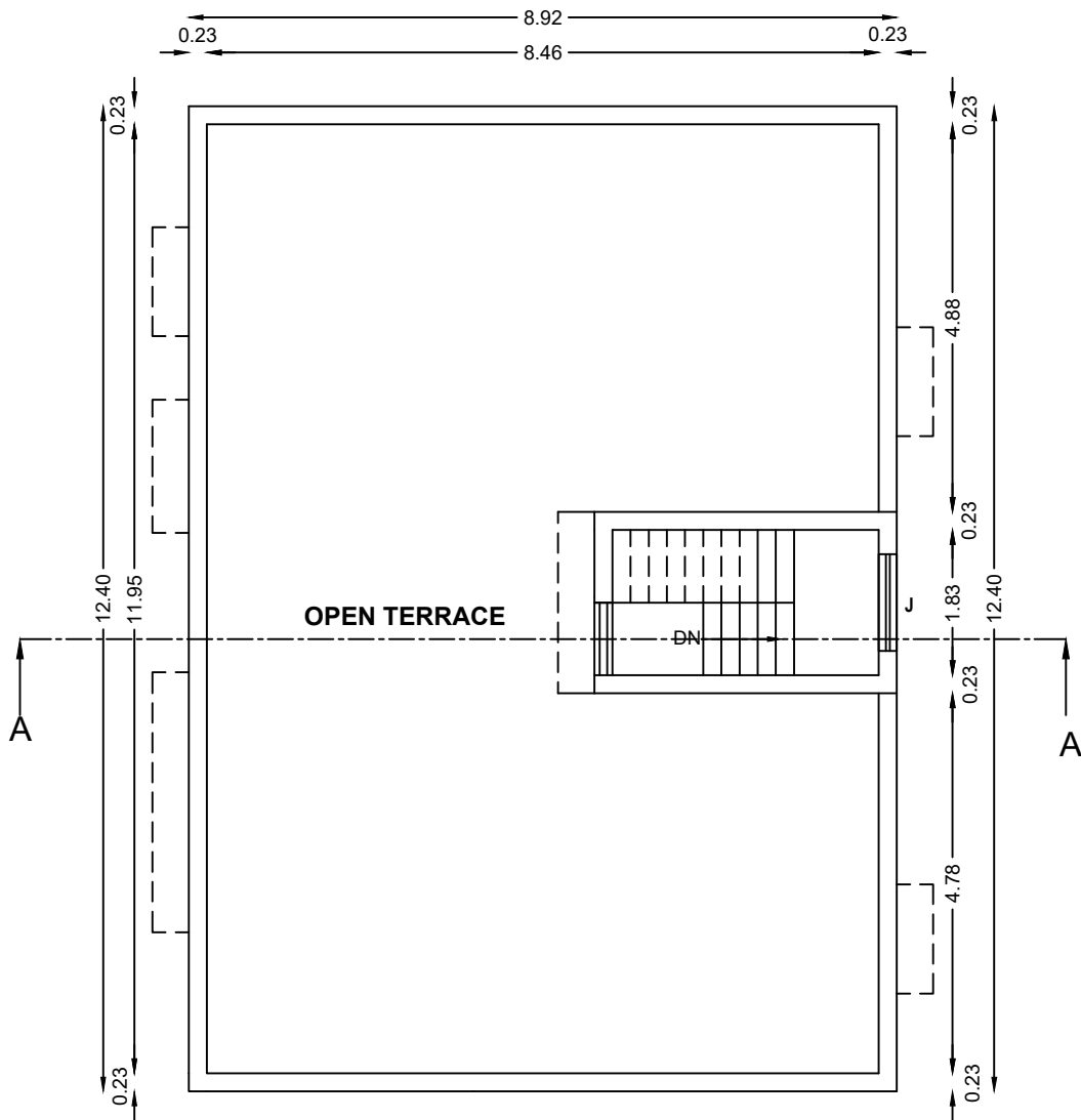
TERRACE PLAN
