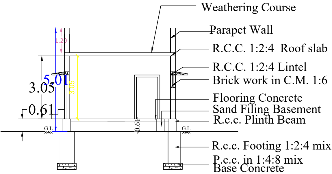
SECTION -"AB"
