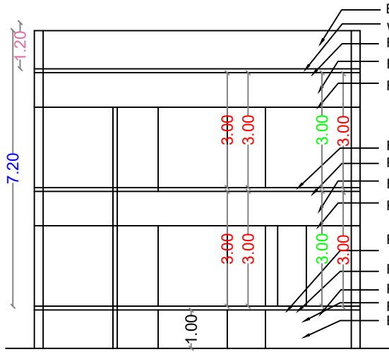
SECTION ON "AA & BB "
