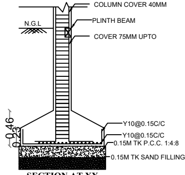
SECTION AT XX
