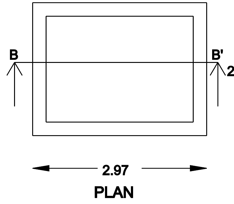
SEPTIC TANK
