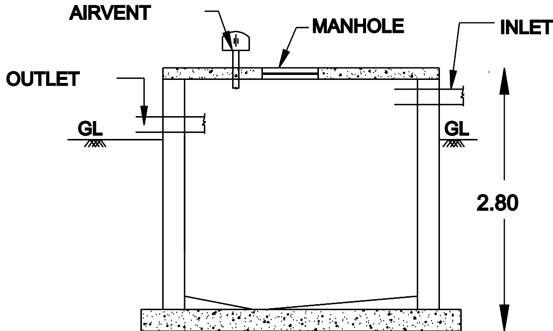
SEPTIC TANK
