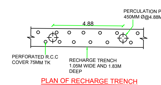
PLAN OF RECHARGE TRENCH
