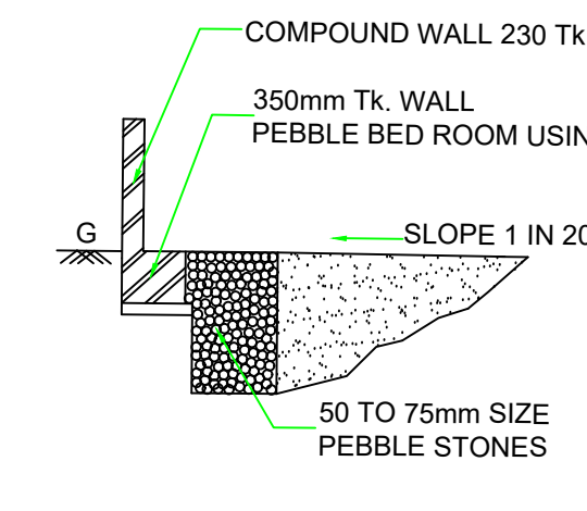
COMPOUND WALL
