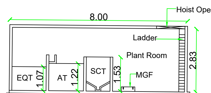
SECTION ON "X-X"
