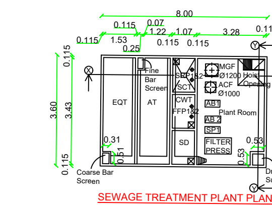
SEWAGE TREATMENT PLANT PLAN
