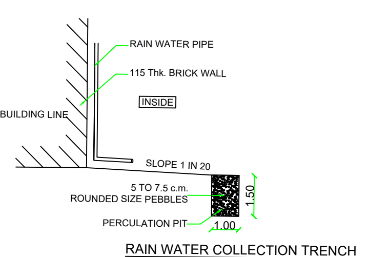
RAIN WATER COLLECTION TRENCH
