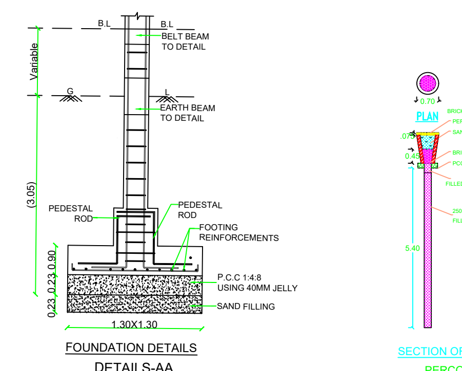
FOUNDATION DETAILS
