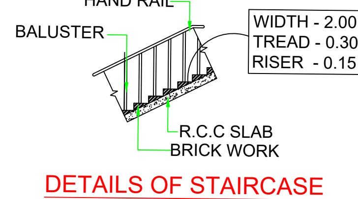
DETAILS OF STAIRCASE
