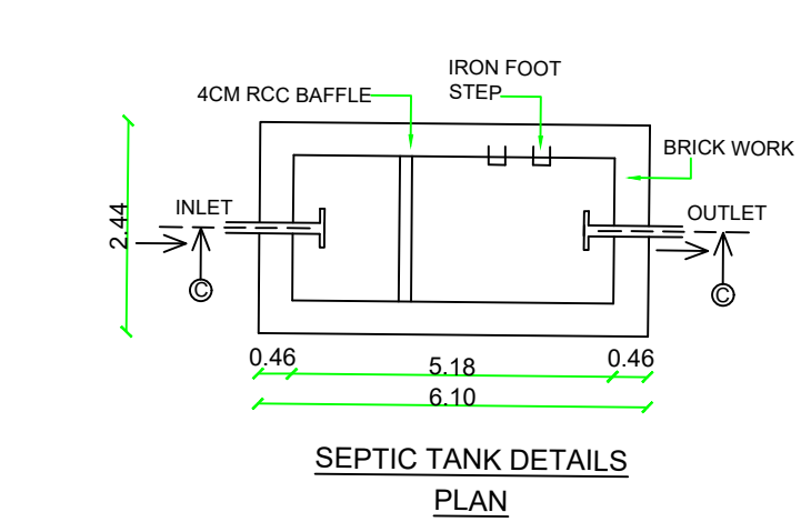
SEPTIC TANK DETAILS PLAN
