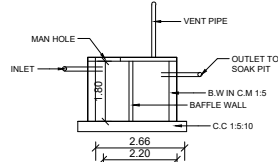
SEPTIC TANK DETAILS
