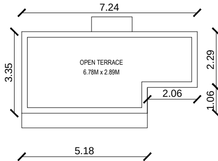
ROOF PLAN
