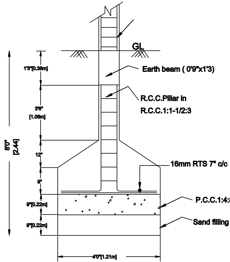
FOUNDATION DETAILS
