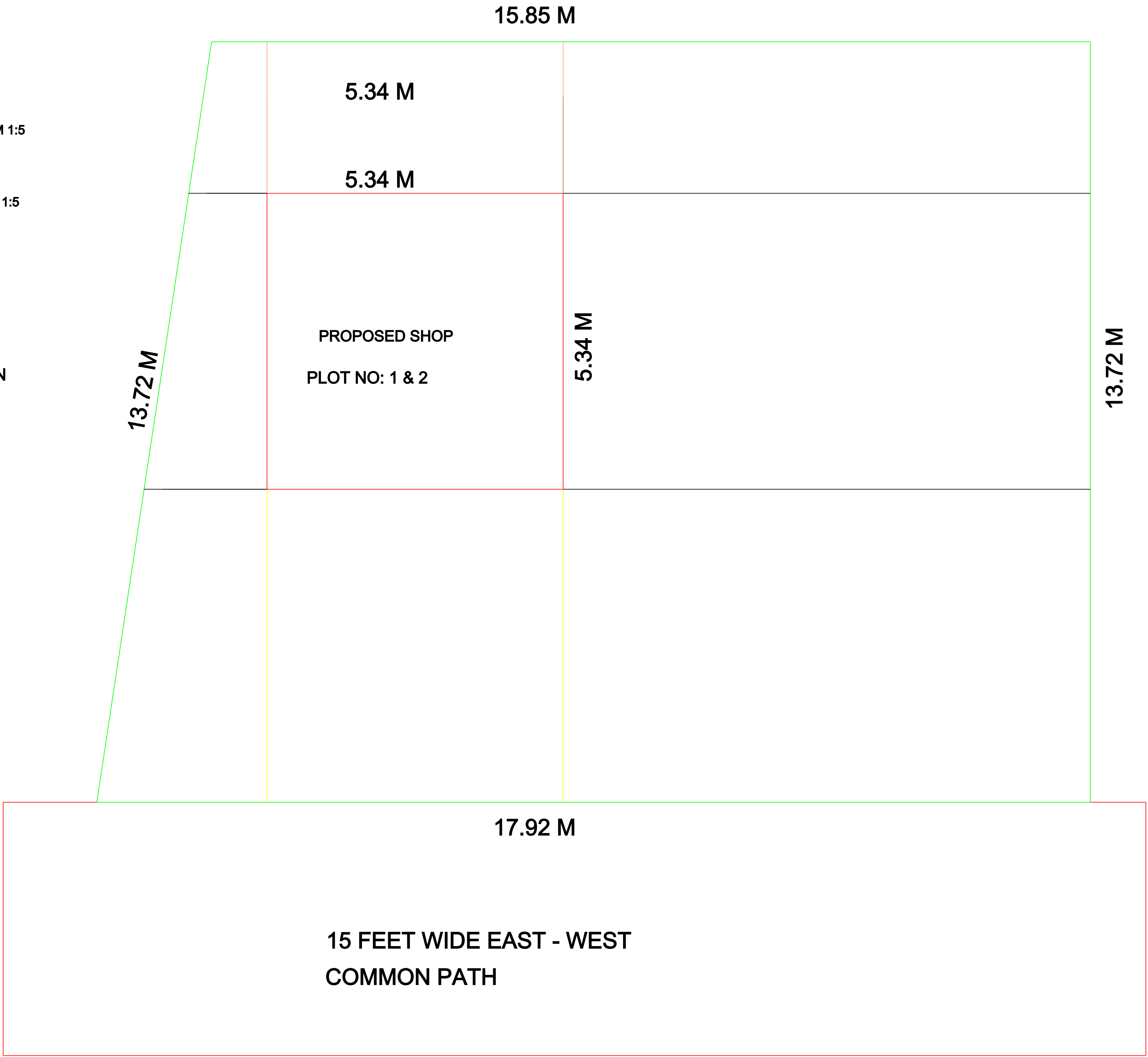
SITE PLAN
