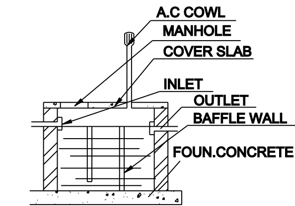
DETAILS OF SEPTIC TANK
