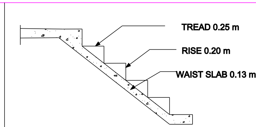
STAIR DETAILS
