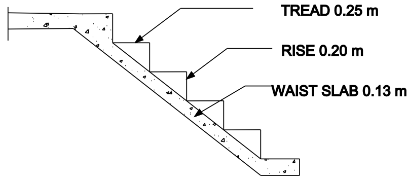
STAIR DETAILS
