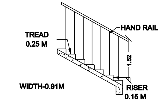
STAIRCASE DETAILS
