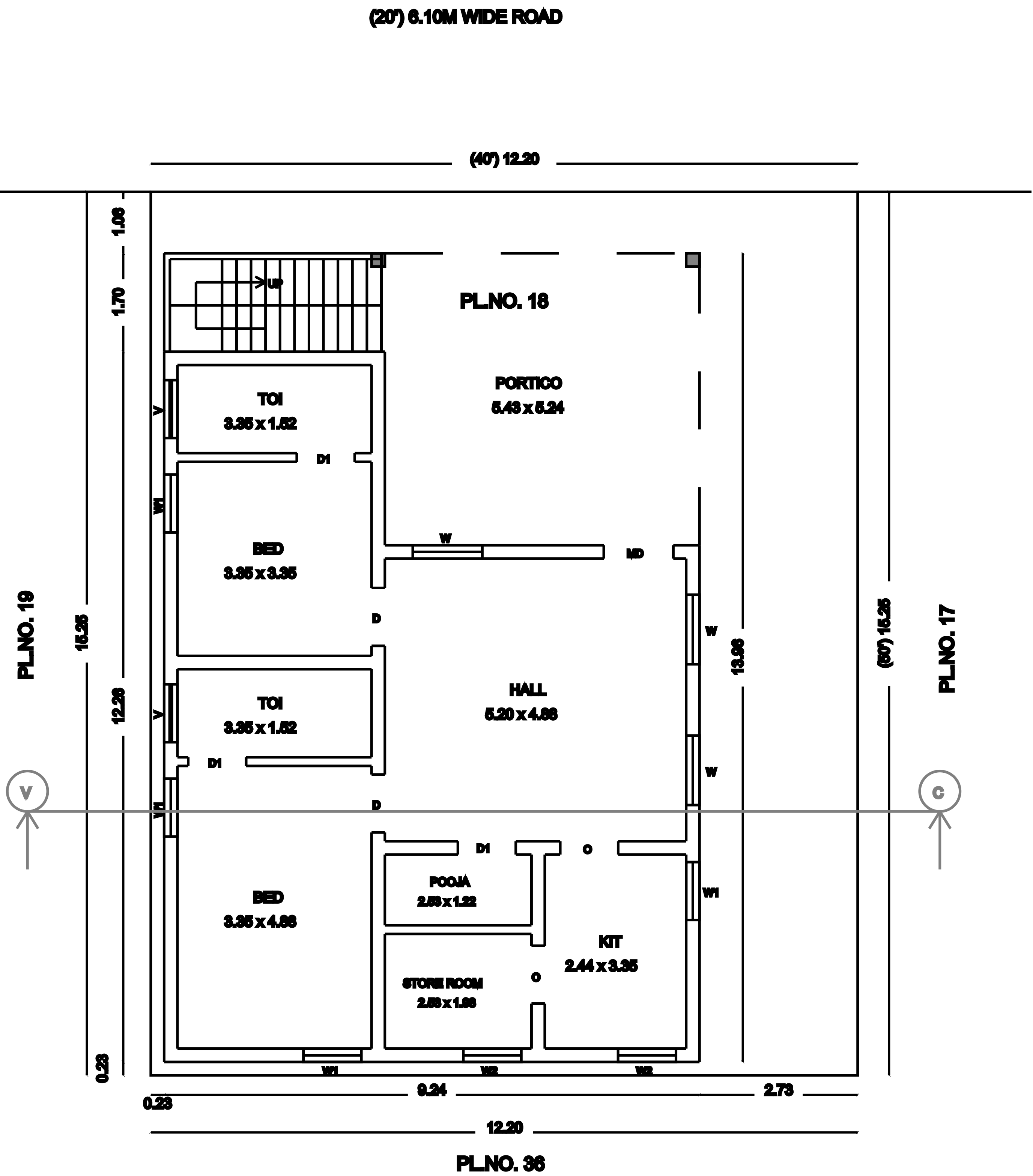
FLOOR PLAN (SCALE :- 1 : 100)
