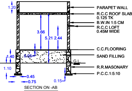
SECTION ON-AB
