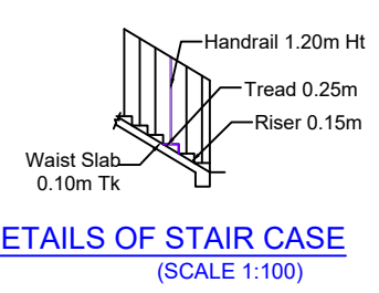
DETAILS OF STAIR CASE (SCALE 1:100)
