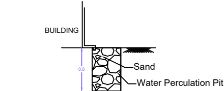
DETAILS OF RAIN WATER PERCOLATION PIT (SCALE 1:100)
