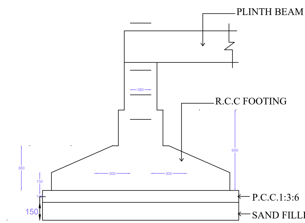
TYPICAL SECTION OF R.C.C. COLUMN FOUNDATION SCALE : 1" = 2'-0"
