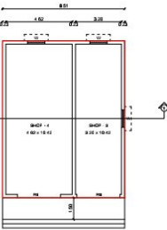
PROPOSED FIRST FLOOR PLAN
