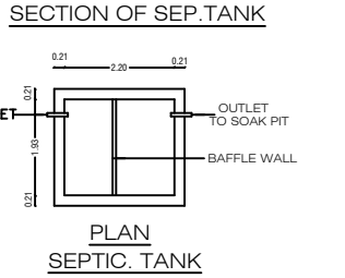
PLAN SEPTIC TANK
