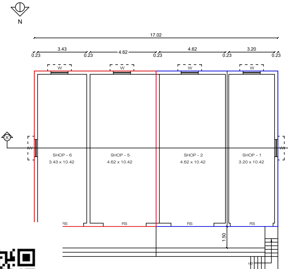
PROPOSED & EXISTING GROUND FLOOR PLAN
