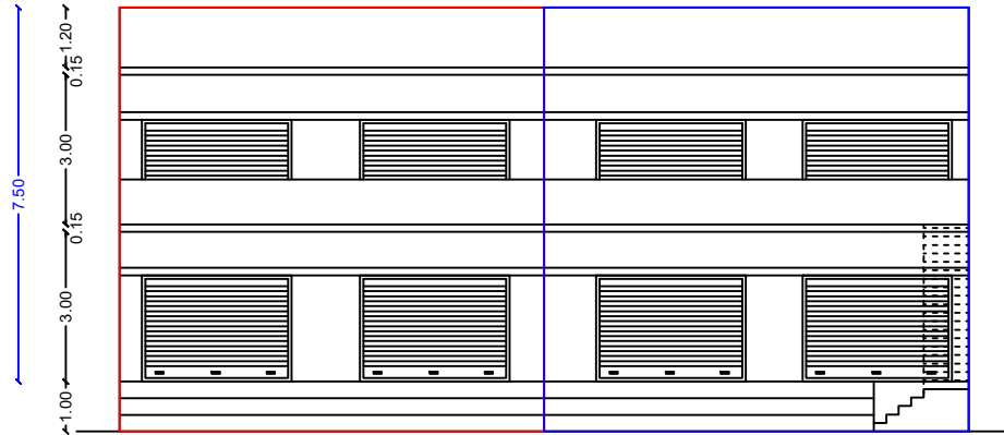
NORTH ELEVATION
