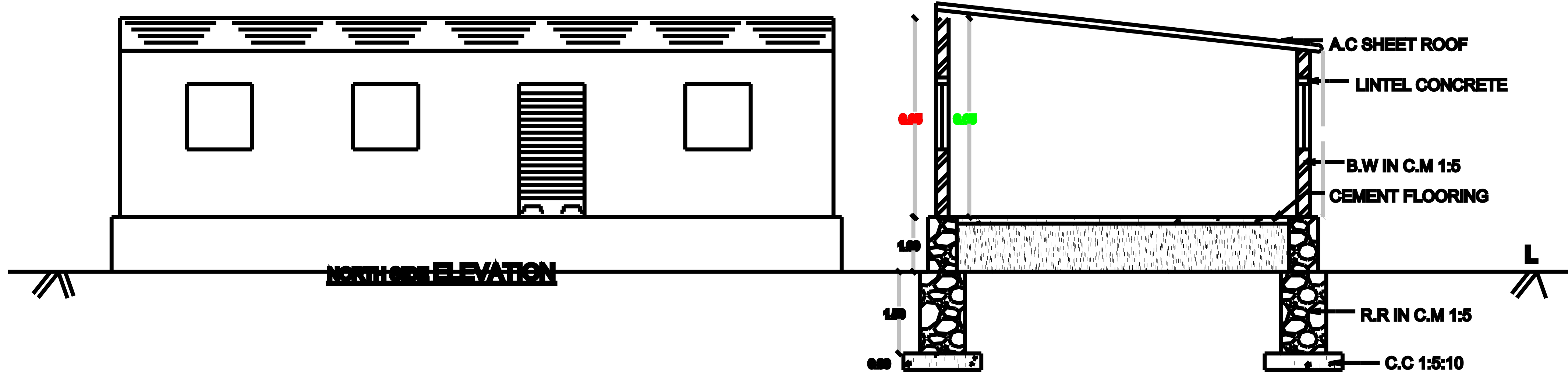
TOILET BLOCK
