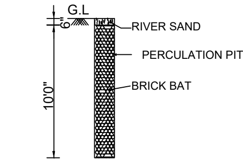
PERCOLATION PIT
