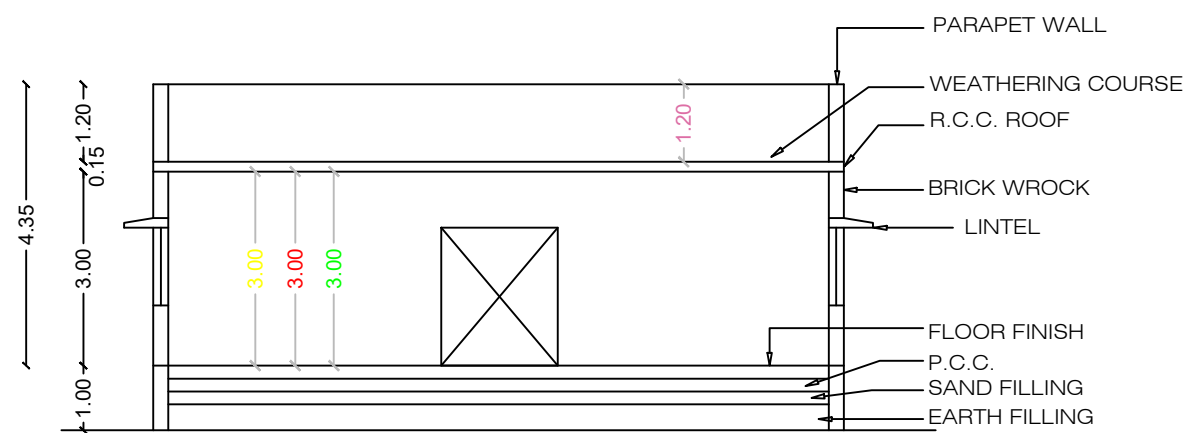
SECTION ON "XY"
