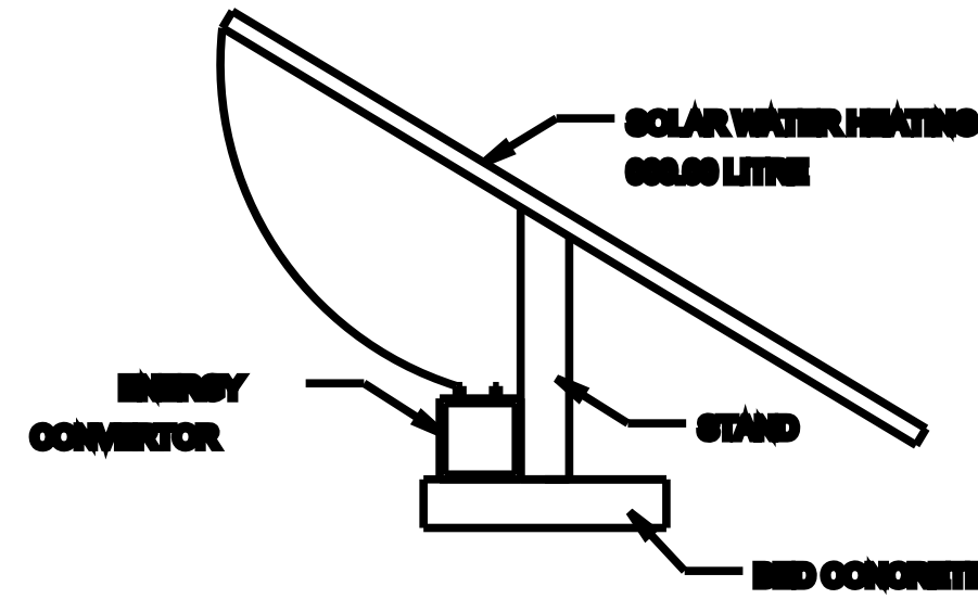
SOLAR SYSTEM
