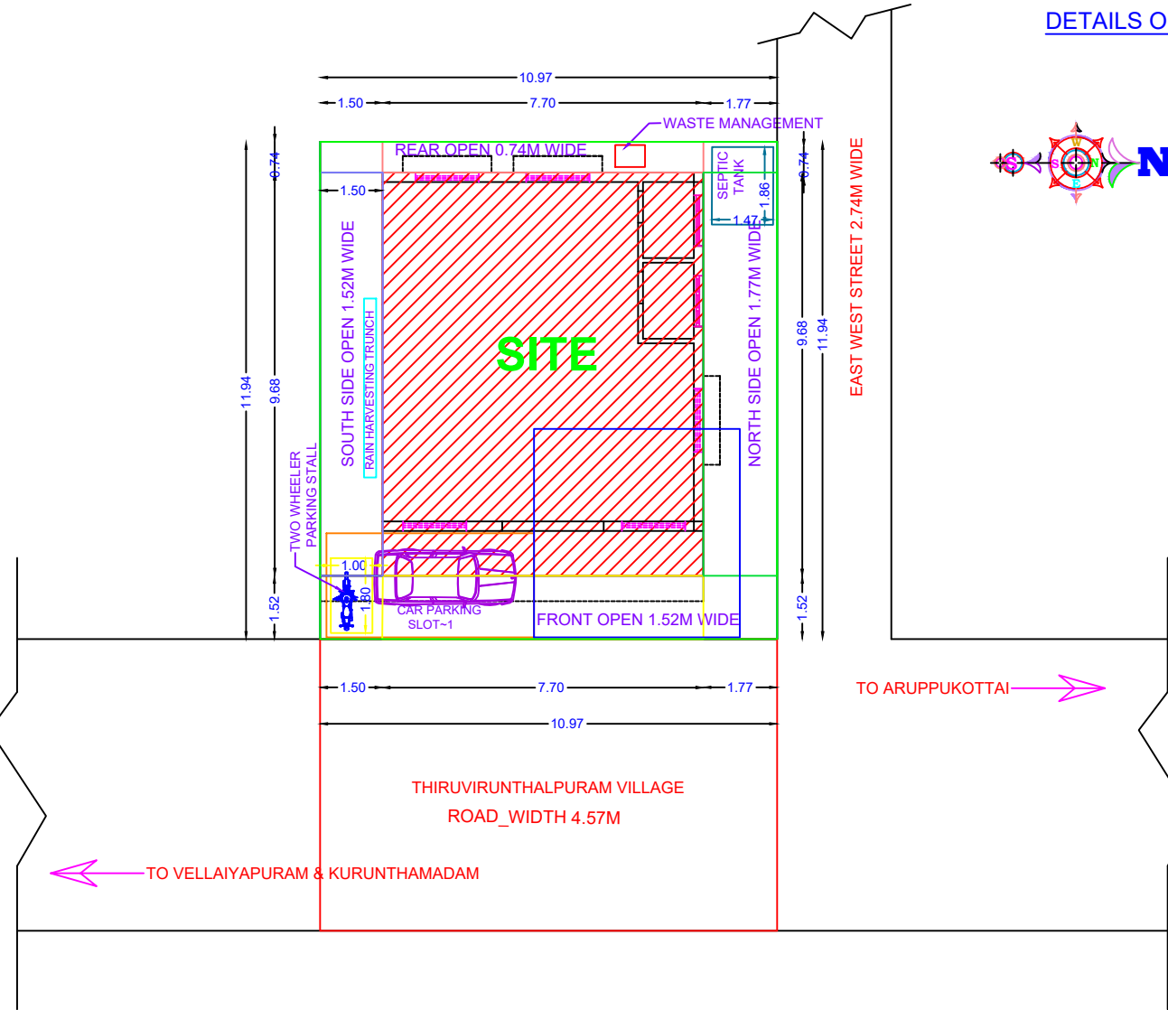
SITE PLAN
