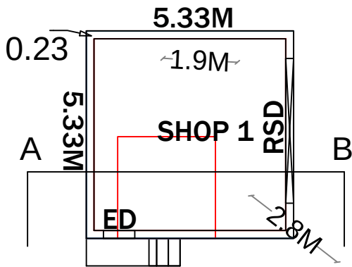
PROPOSED GROUND FLOOR PLAN,1:100
