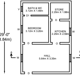
EXISTING GROUND FLOOR
