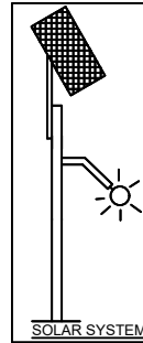
SOLAR SYSTEM
