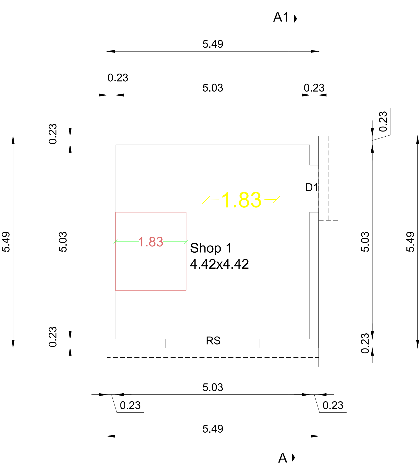
GROUND FLOOR PLAN BLOCK - 1
