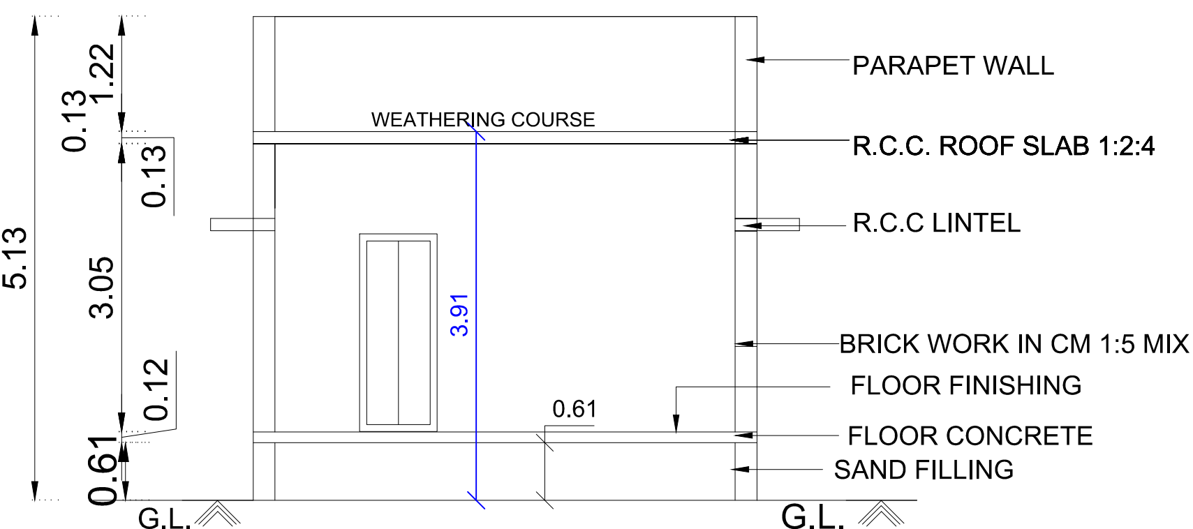
SECTION A-A1 BLOCK - 1
