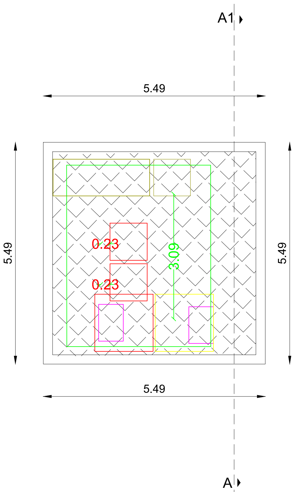
TERRACE FLOOR PLAN BLOCK - 2
