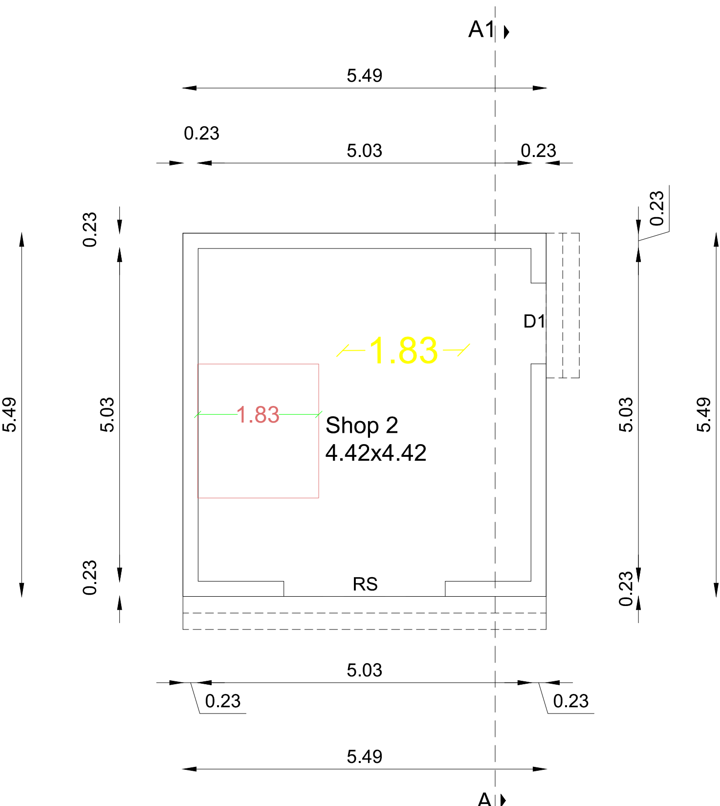
GROUND FLOOR PLAN BLOCK - 2
