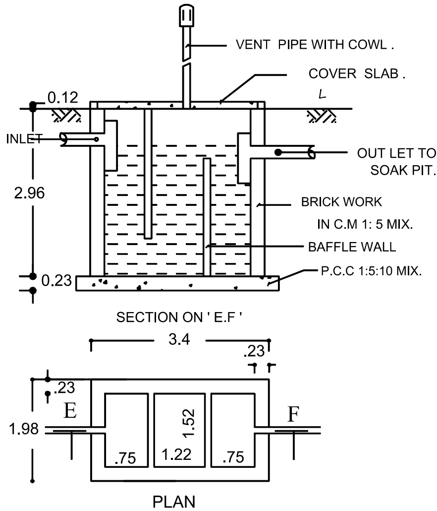
SEPTIC TANK DETAILS ( NOT TO SCALE )
