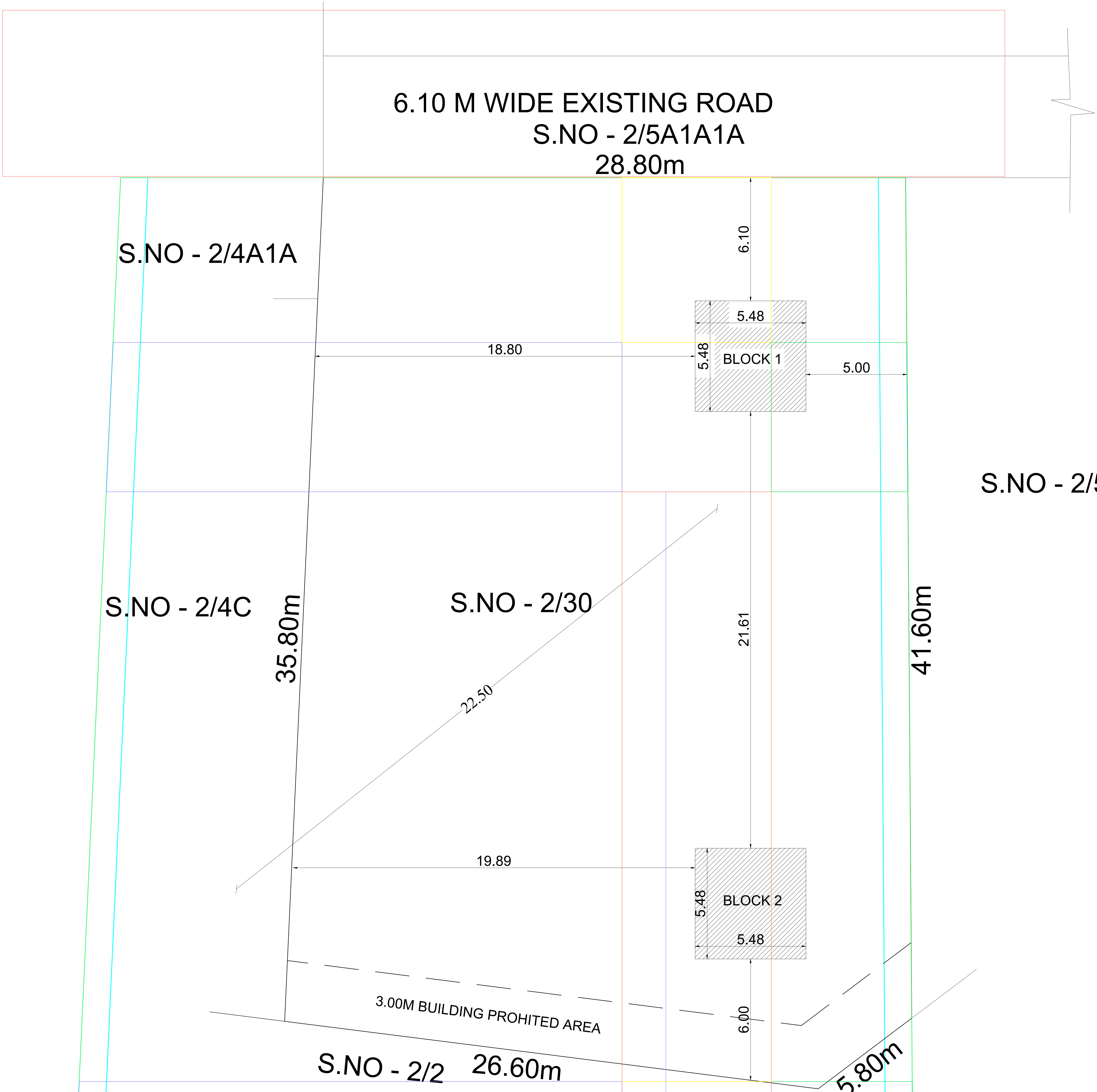
SITE PLAN
