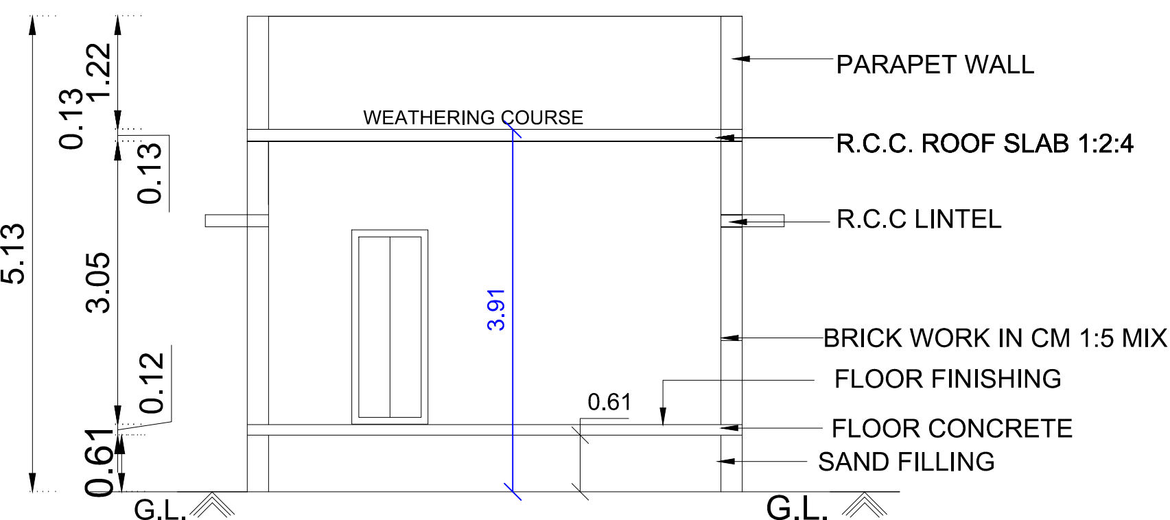
SECTION A-A1 BLOCK - 2
