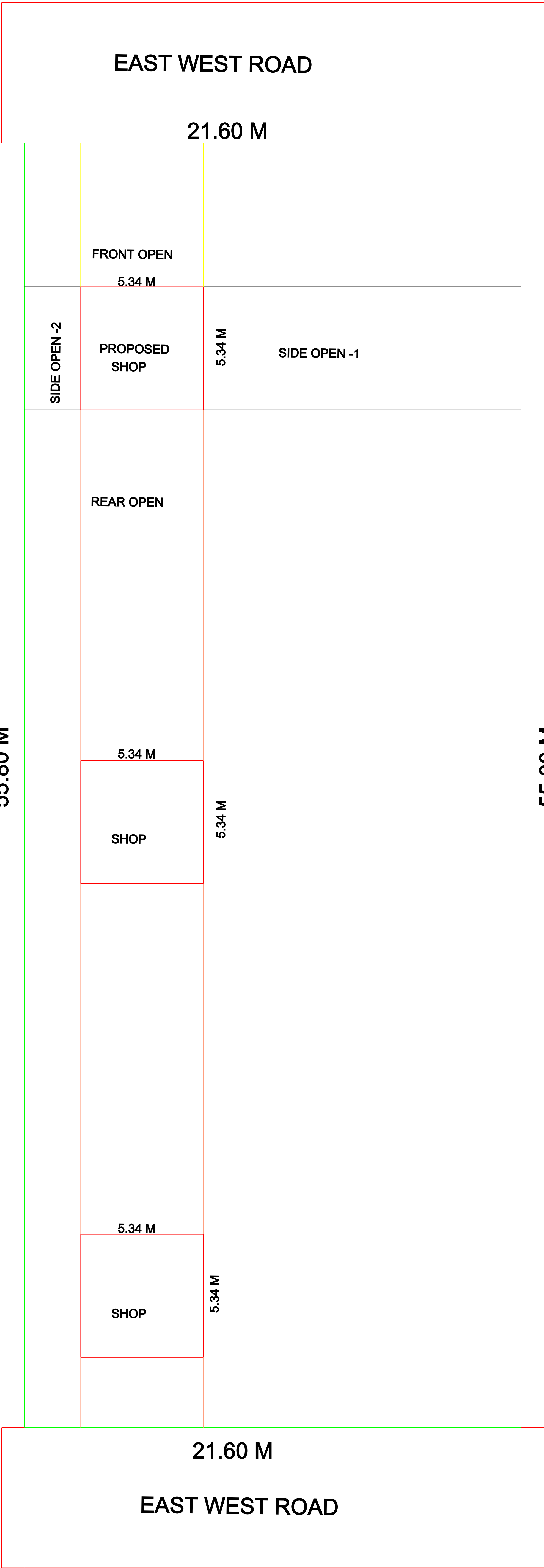
SITE PLAN
