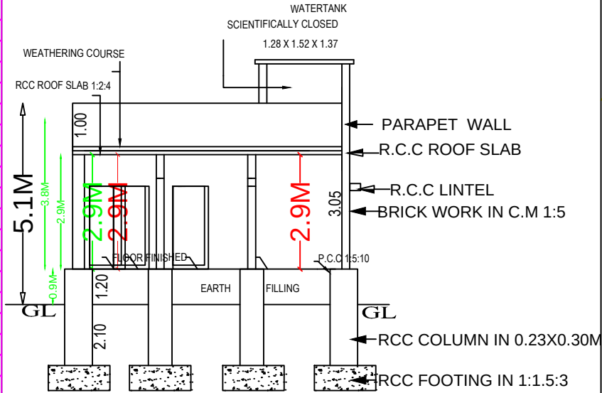
SECTION "A-B"
