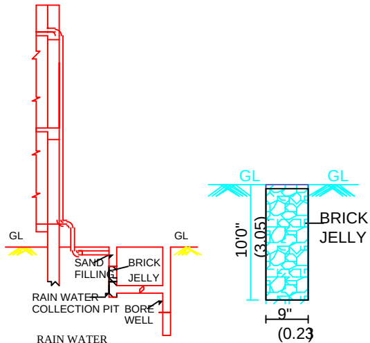
PERCOLATION PIT
